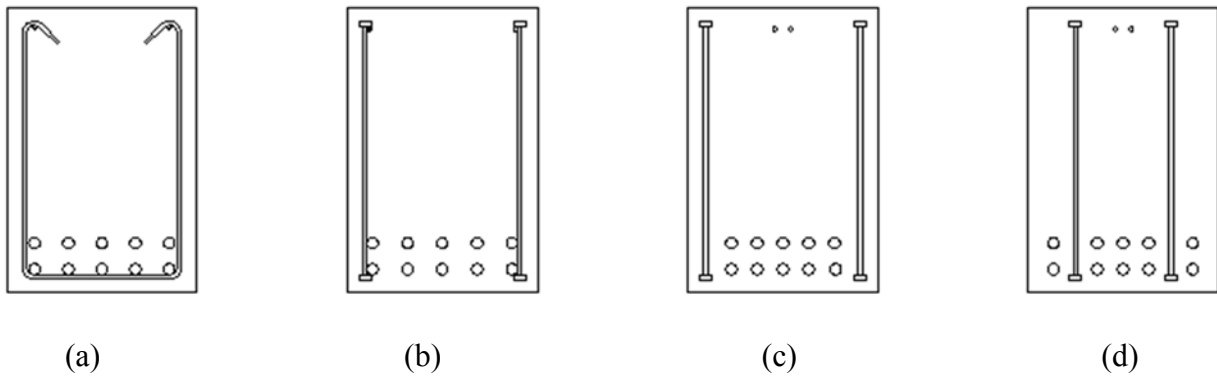
Figure 2.1: Transverse reinforcement configurations: (a) conventional U-shaped hooked stirrup (S), (b) headed bars engaged (HE), (c) headed bars not engaged (HNE), (d) headed bars within longitudinal reinforcement not engaged (HNE2)
