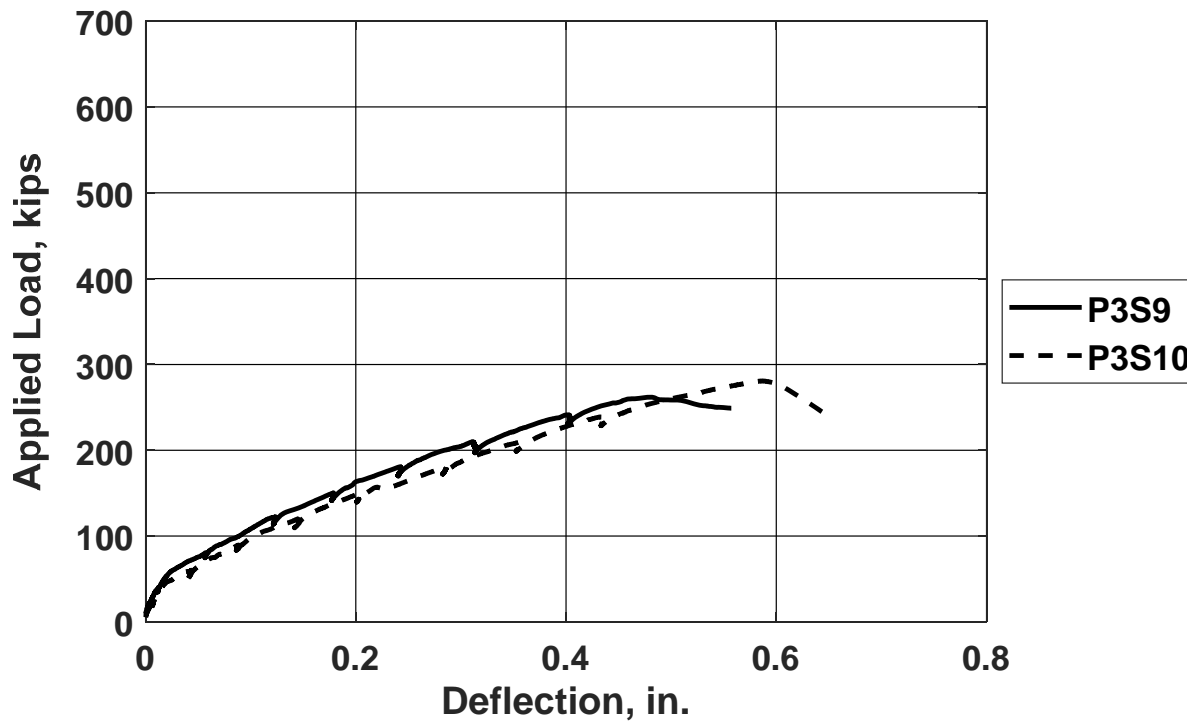
Figure F.17: Load versus deflection for specimens P3S9 and P3S10 (SM1 was missing for specimen P3S9; SM2 data were used to represent beam settlement at supports) [1 kip = 4.45 kN, 1 in. = 25.4 mm]
