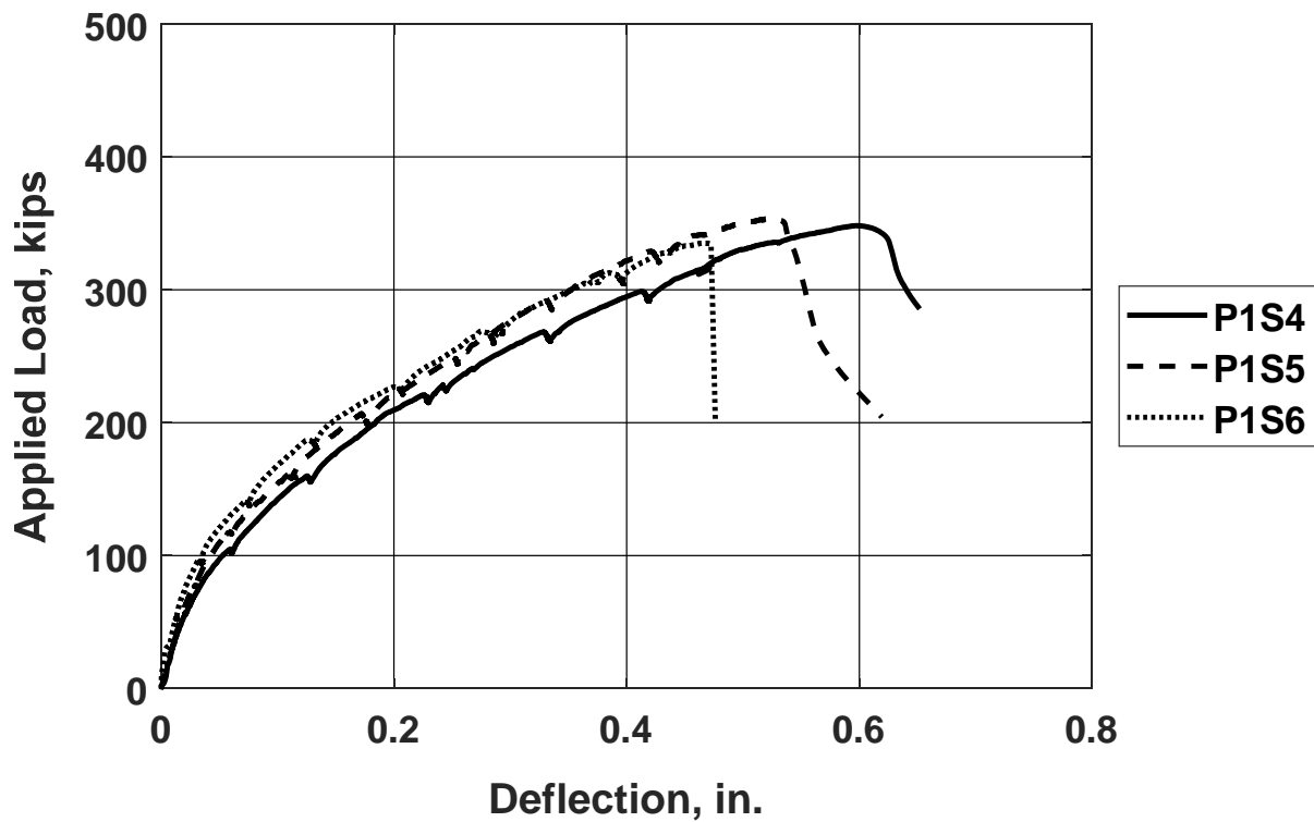
Figure F.3: Load versus deflection for specimens P1S4 through P1S6 [1 kip = 4.45 kN, 1 in. = 25.4 mm]
