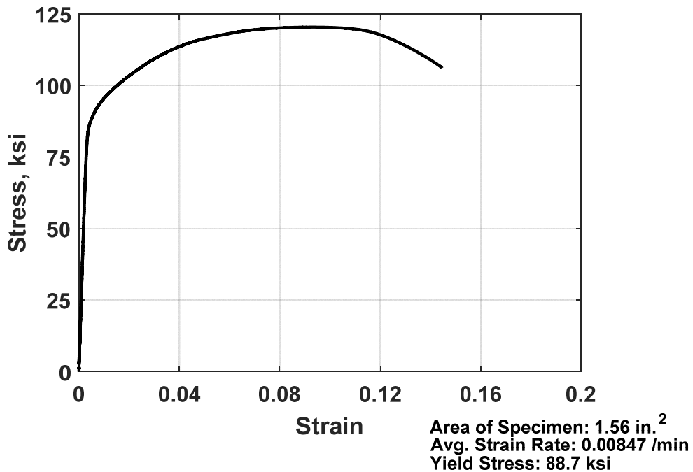
Figure D.7: Stress versus strain for No. 11 [No. 36] longitudinal reinforcing bar (Grade 80 [Grade 550], Sample 1, Phase 1) [1 in. 2 = 0.000645 m 2 , 1 ksi = 6.9 MPa]
