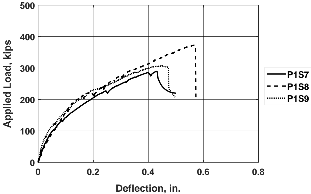
Figure F.4: Load versus deflection for specimens P1S7 through P1S9 [1 kip = 4.45 kN, 1 in. = 25.4 mm]
