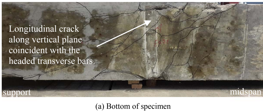
Figure 3.5: Damage to specimen P1S15 ( f_{ym} = 85.0 ksi [587 MPa], h = 36 in. [910 mm], HNE detail)
