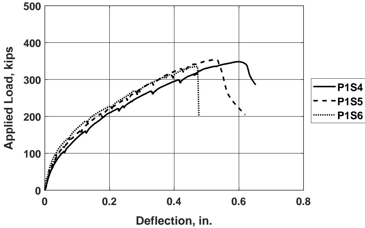
Figure 3.7: Applied load versus midspan deflection for specimens P1S4 through P1S6 ( f_{ym} = 69.8 ksi [482 MPa], \rho f_{ym} = 96.9 psi [669 kPa], h = 36 in. [910 mm], f_{cm} = 4240 to 4360 psi [29.3 to 30.1 MPa]) [1 in. = 25.4 mm, 1 kip = 4.45 kN]
