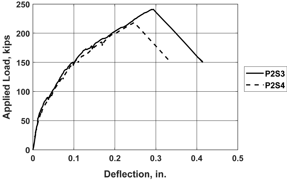
Figure F.8: Load versus deflection for specimens P2S3 and P2S4 (SM2 was missing for both specimens; SM1 data were used to represent beam settlement at supports) [1 kip = 4.45 kN, 1 in. = 25.4 mm]
