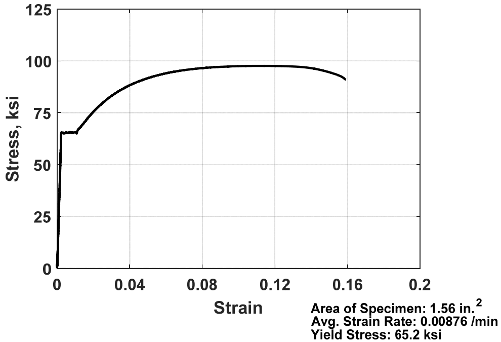
Figure D.20: Stress versus strain for No. 11 [No. 36] longitudinal reinforcing bar (Grade 60 [Grade 420], Sample 2, Phase 2) [1 in. 2 = 0.000645 m 2 , 1 ksi = 6.9 MPa]
