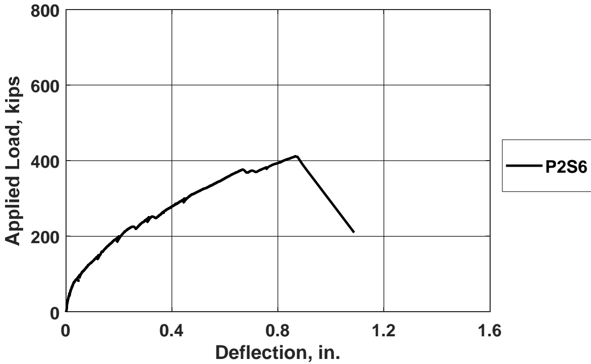
Figure F.9: Load versus deflection for specimen P2S6 (deflection data not obtained for specimen P2S5) [1 kip = 4.45 kN, 1 in. = 25.4 mm]
