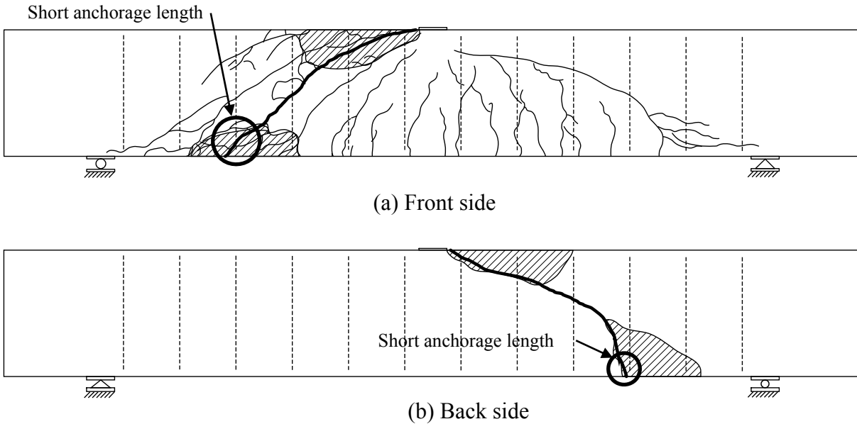
Figure 3.24: Damage to specimen P1S1
