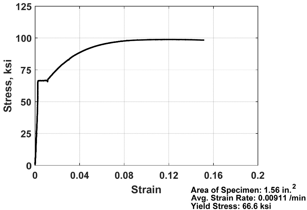
Figure D.19: Stress versus strain for No. 11 [No. 36] longitudinal reinforcing bar (Grade 60 [Grade 420], Sample 1, Phase 2) [1 in. 2 = 0.000645 m 2 , 1 ksi = 6.9 MPa]
