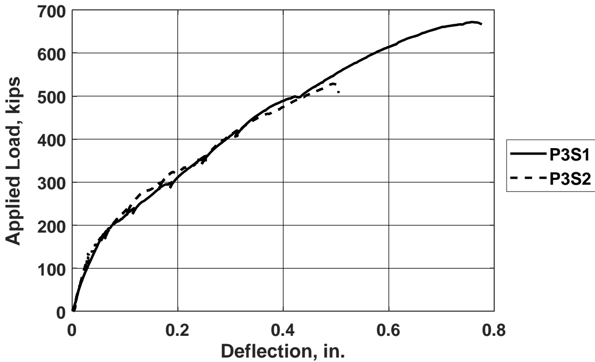
Figure F.13: Load versus deflection for specimens P3S1 and P3S2 [1 kip = 4.45 kN, 1 in. = 25.4 mm]
