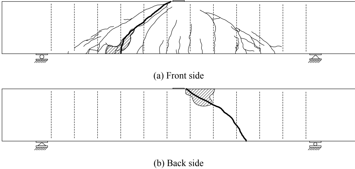
Figure 3.5: Damage to specimen P1S15 ( f_{ym} = 85.0 ksi [587 MPa], h = 36 in. [910 mm], HNE detail)
