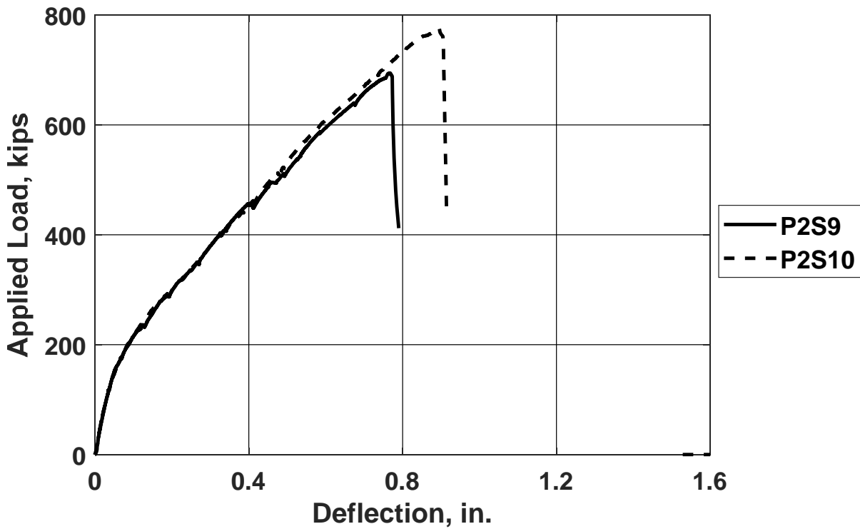
Figure F.11: Load versus deflection for specimens P2S9 and P2S10 [1 kip = 4.45 kN, 1 in. = 25.4 mm]
