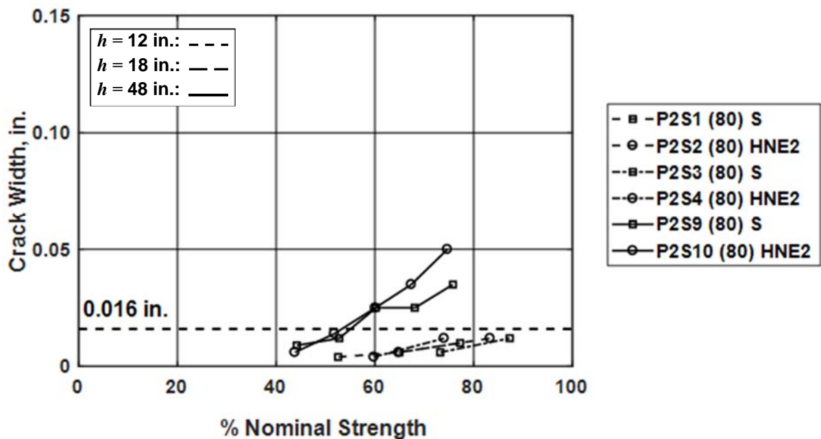
Figure 3.18: Maximum crack width versus percent of nominal strength: specimens with h = 12, 18, and 48 in. [1 in. = 25.4 mm]
