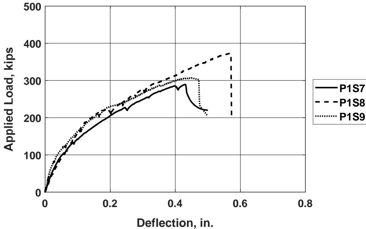
Figure 3.8: Applied load versus midspan deflection for specimens P1S7 through P1S9 ( f_{ym} = 85.0 ksi [587 MPa], \rho_{fym} = 88.5 psi [610 kPa], h = 36 in. [910 mm], f_{cm} = 4110 to 5260 psi [28.4 to 36.3 MPa]) [1 in. = 25.4 mm, 1 kip = 4.45 kN]
