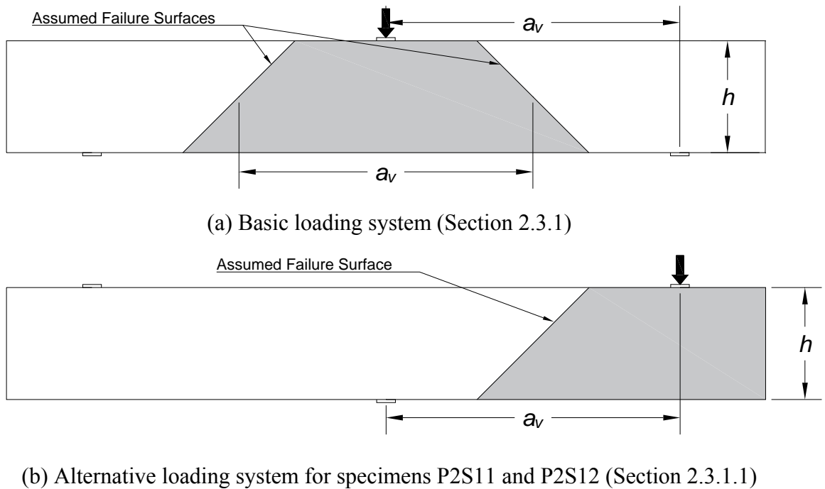
Figure 3.10: Assumed failure surfaces and self-weight considered in shear strength (shaded)
