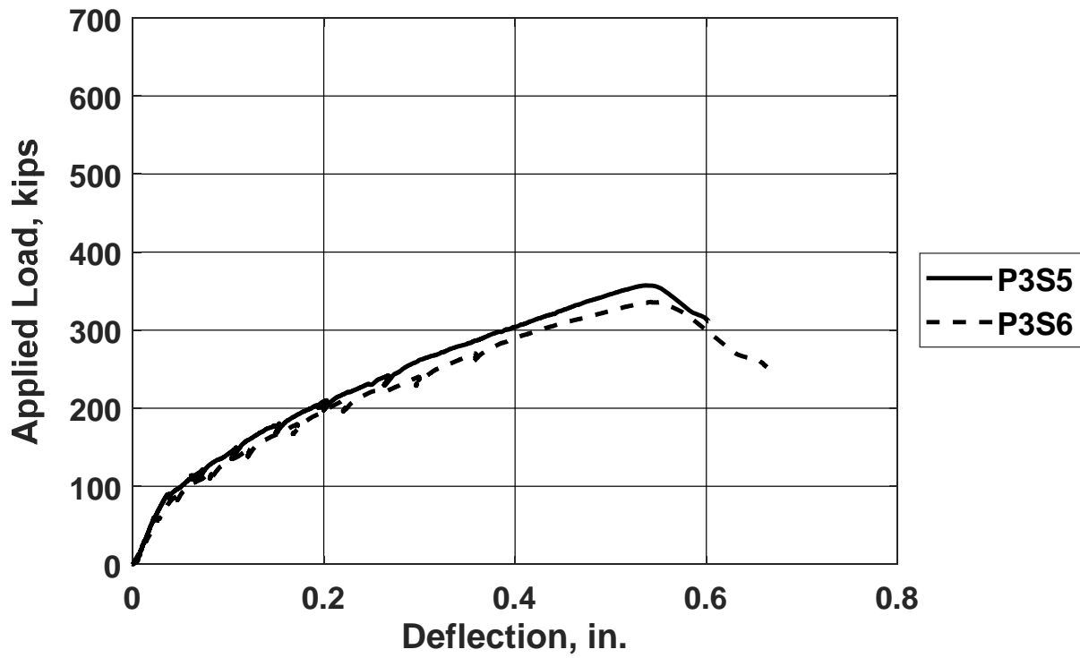
Figure F.15: Load versus deflection for specimens P3S5 and P3S6 [1 kip = 4.45 kN, 1 in. = 25.4 mm]
