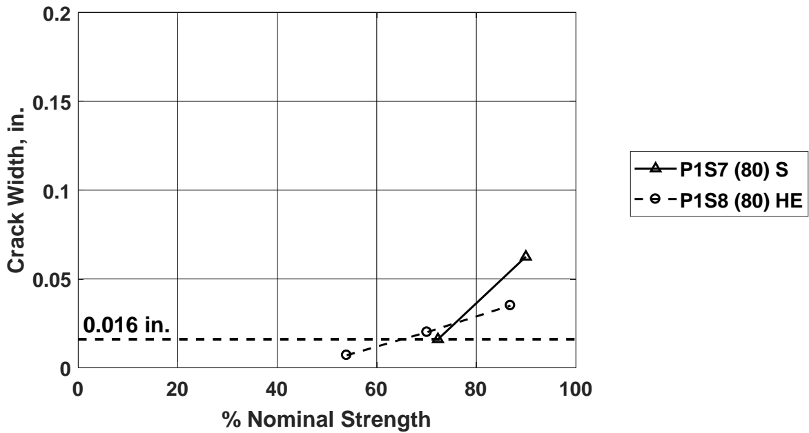
Figure G.5: Crack width versus percent of nominal strength: specimens P1S7 and P1S8 [1 in. = 25.4 mm]
