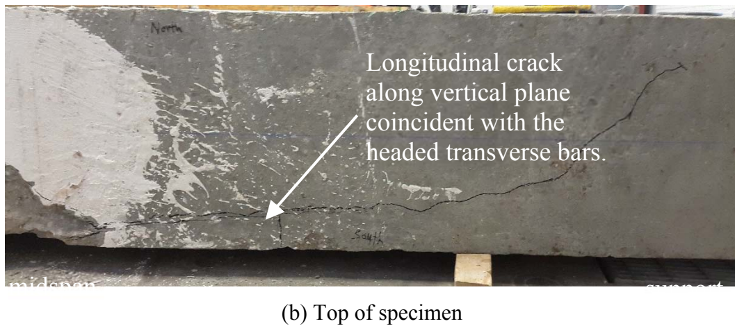
Figure 3.6: Damage observed on back side of specimen P1S15 ( f_{ym} = 85.0 ksi [587 MPa], h = 36 in. [910 mm], HNE detail)
