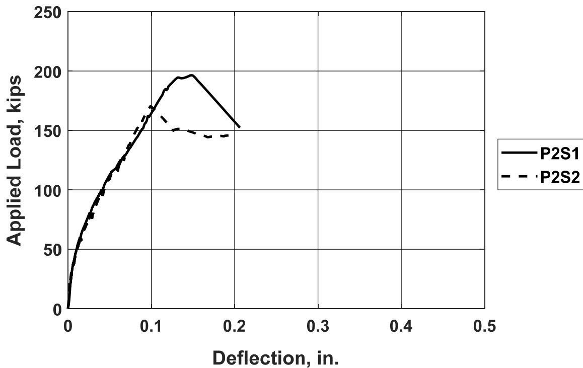
Figure F.7: Load versus deflection for specimens P2S1 and P2S2 (SM1 and SM2 were both missing for both specimens; the average vertical displacement of markers A1 and B1 was used to represent beam settlement at supports) [1 kip = 4.45 kN, 1 in. = 25.4 mm]
