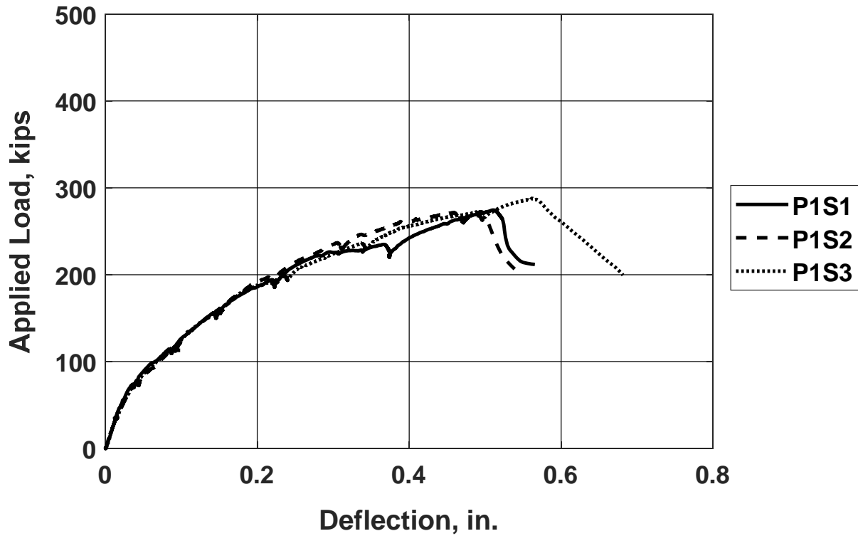
Figure F.2: Load versus deflection for specimens P1S1 through P1S3 [1 kip = 4.45 kN, 1 in. = 25.4 mm]
