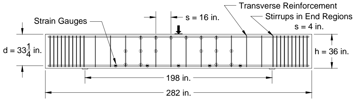
Figure B.21: Elevation of P3S1 through P3S4 [1 ksi = 6.9 MPa, 1 in. = 25.4 mm]
