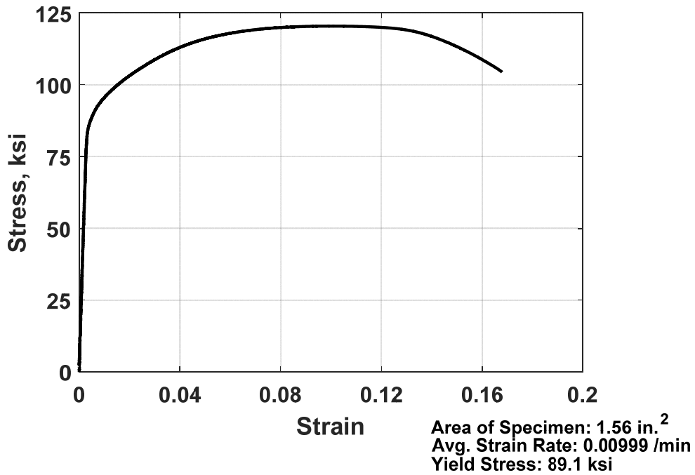
Figure D.8: Stress versus strain for No. 11 [No. 36] longitudinal reinforcing bar (Grade 80 [Grade 550], Sample 2, Phase 1) [1 in. 2 = 0.000645 m 2 , 1 ksi = 6.9 MPa]
