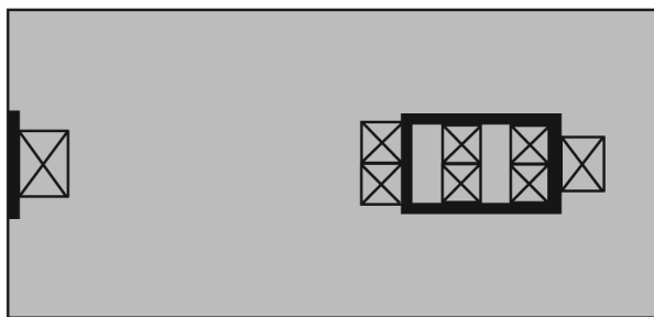
Figure 6.6 Illustration of diaphragms with limited connectivity to vertical elements of the seismic-force-resisting system.
