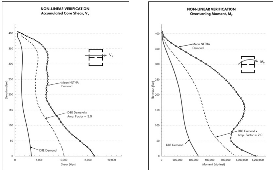
Figure 6.7 Higher-mode effects on shear and flexural demand distributions in a tall core-wall building.
